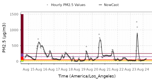
Hourly PM2.5 Values and NowCast Site: Unit67
