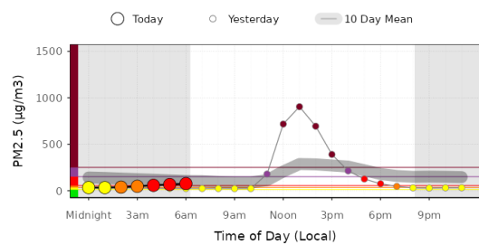
NowCast by Time of Day Site: Unit67
