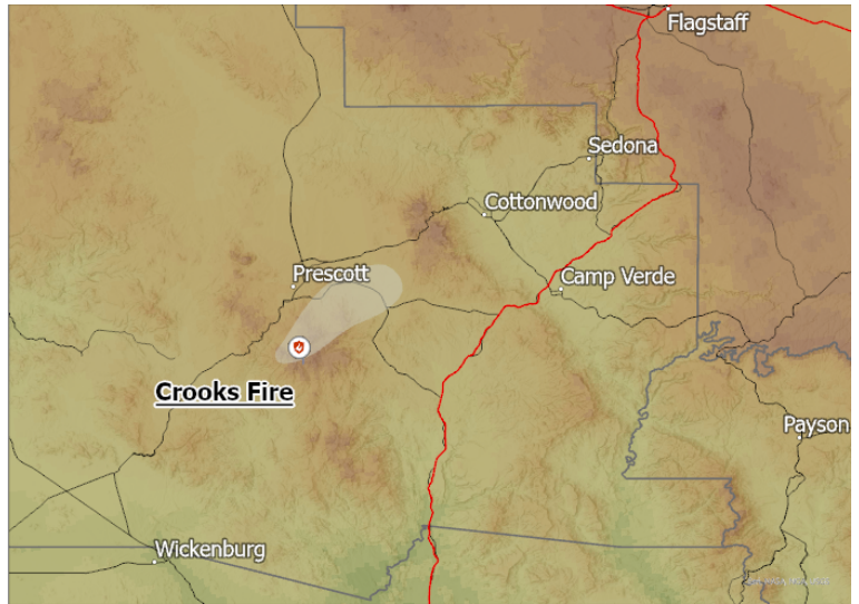
SMOKE PLUME TRAJECTORY FOR: May 01, 2022 Use graphic for reference only
